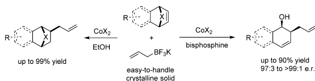
Scheme 1. Unprecedented cobalt-catalyzed allylation of heterobicyclic alkenes.
