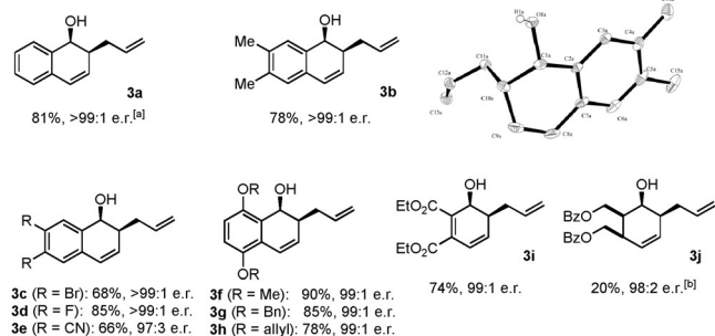
b) Regiodivergent allylative ring opening
