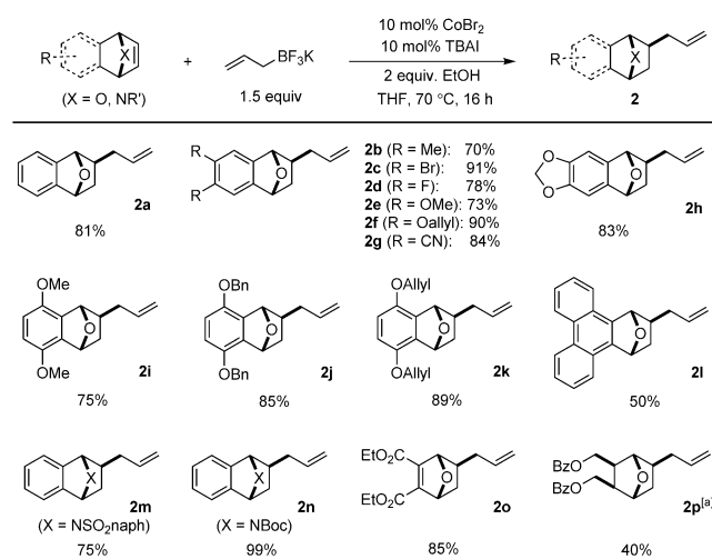
Scheme 2. Scope of cobalt-catalyzed hydroallylation. See the Supporting Information for a detailed procedure. [a] 30 mol % CoBr 2 . Boc = tert -butoxycarbonyl, Bz = benzoyl, TBAI = tetra- n -butylammonium iodide.
